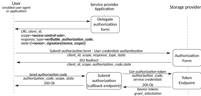
Fig. 5. Verifiable authorization code for extended OAuth2
