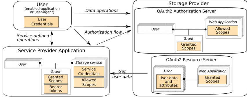
Fig. 2. OAuth2 architecture in the user-centric scenario
