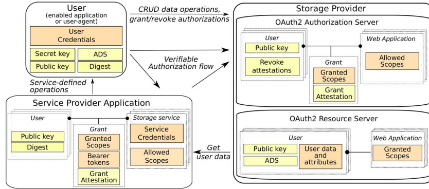
Fig. 4. Architecture for verifiable delegated authorization
